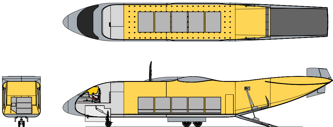
SM-100 PAYLOAD CONFIGURATION With Five LD-3 Containers
