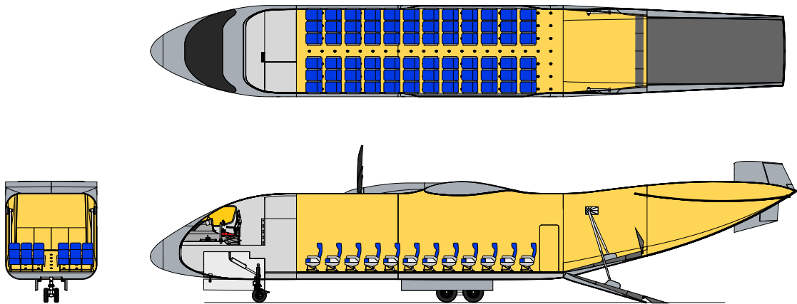
SM-100 PAYLOAD CONFIGURATION With 72 Economy (17 in) Seats @ 31 in Pitch
