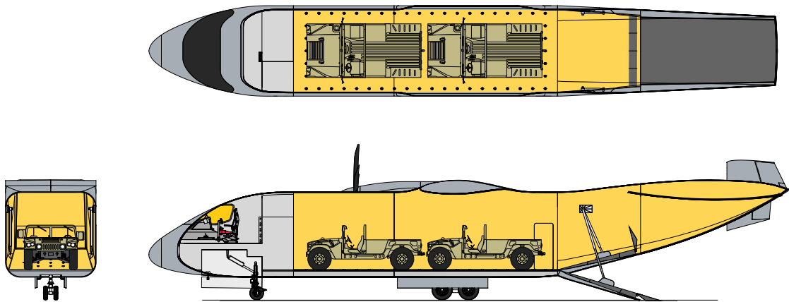
SM-100 PAYLOAD CONFIGURATION With Two HUMVEES
