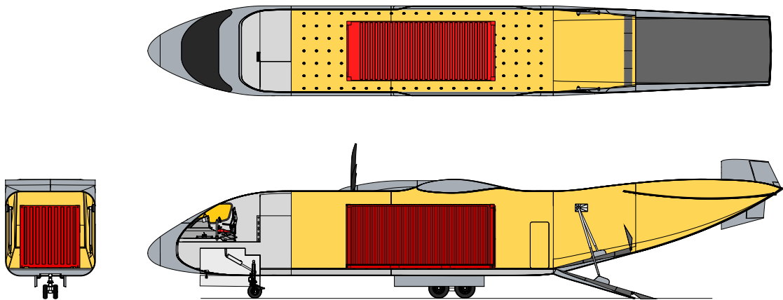
SM-100 PAYLOAD CONFIGURATION With 20 ft x 8 ft x 8 ft SeaLand Container
