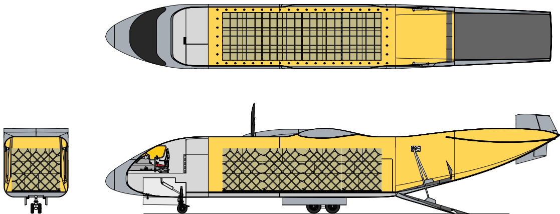
SM-100 PAYLOAD CONFIGURATION With Four 486L Pallets
