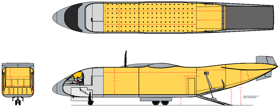
SM-100 PAYLOAD CONFIGURATION General Dimensions
